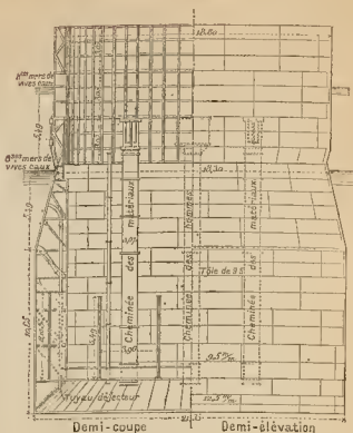
Fig. 2. Cajones Queensferry
